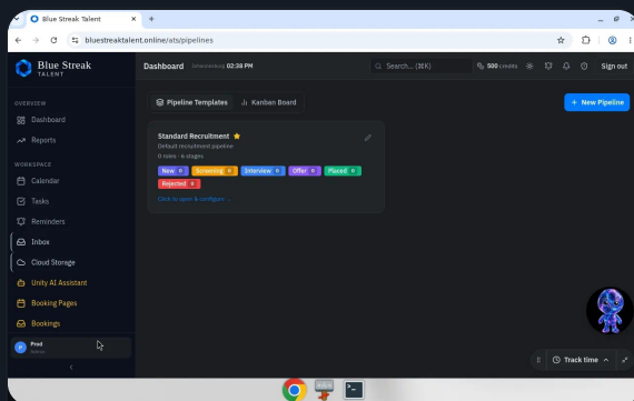
Pipelines
