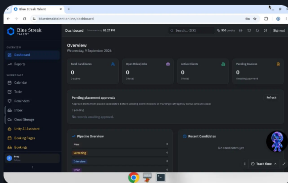
Dashboard
