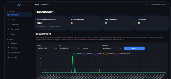
Mailer dashboard
