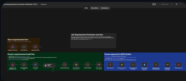
Job requirements
