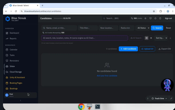
Candidates
